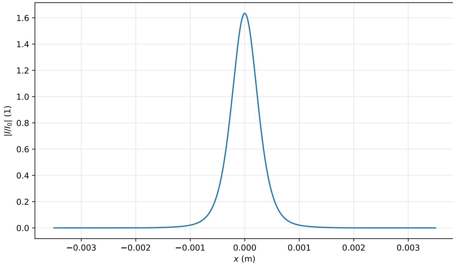
Intensity profile I(x, y = 0, z = 2.070m)/I_0 , P_{in}=0.9P_{cr} , artificial time
